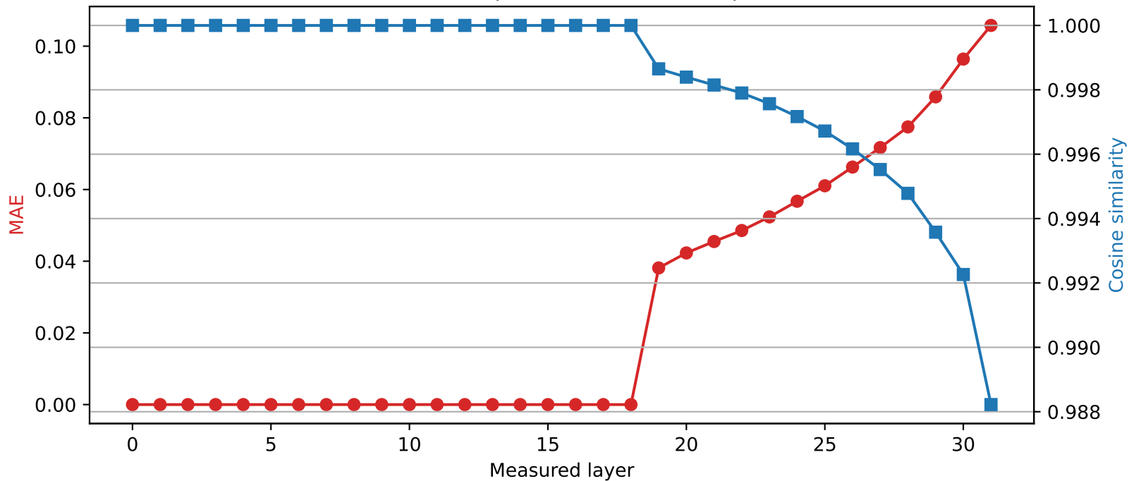
Mistral-7B-Instruct-v0.3 | Quantized layer 18 | float64 \rightarrow int2
