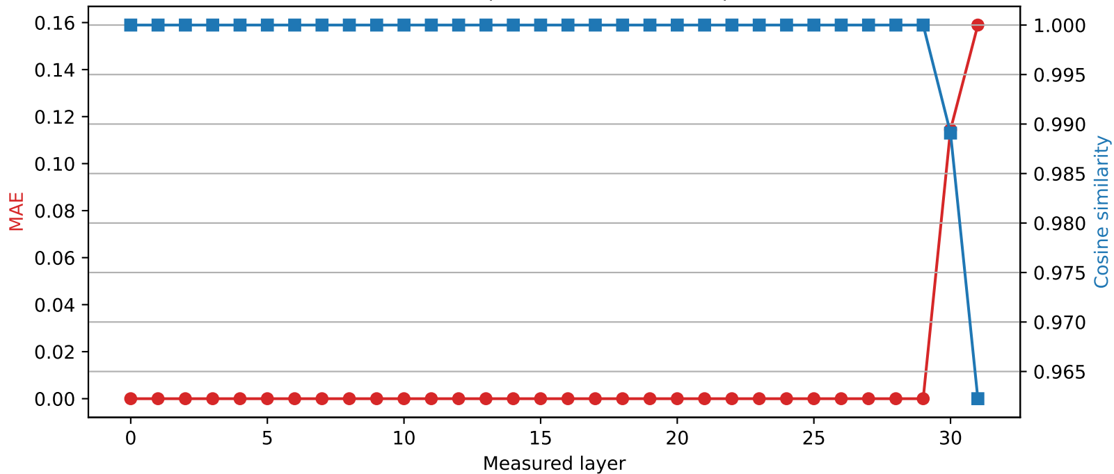
Mistral-7B-Instruct-v0.3 | Quantized layer 29 | float64 \rightarrow int2
