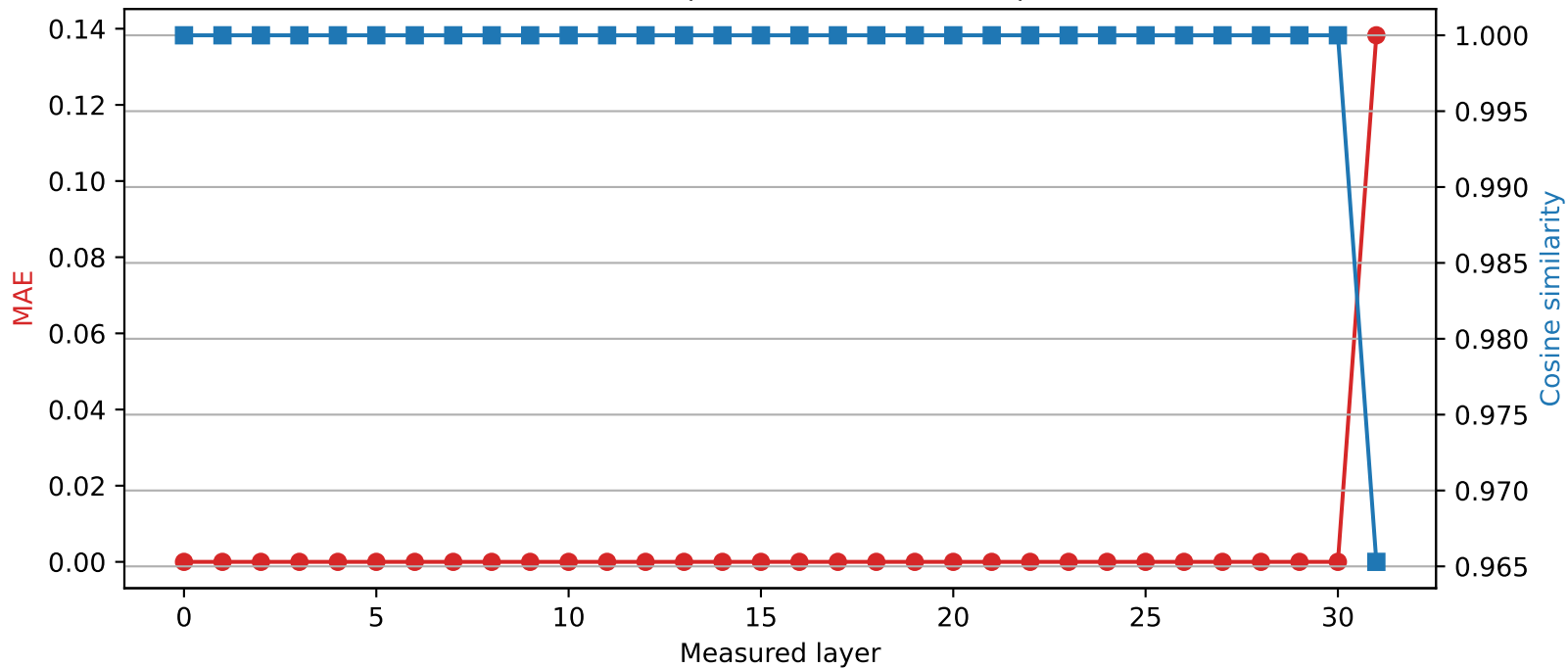
Mistral-7B-Instruct-v0.3 | Quantized layer 30 | float64 \rightarrow int2
