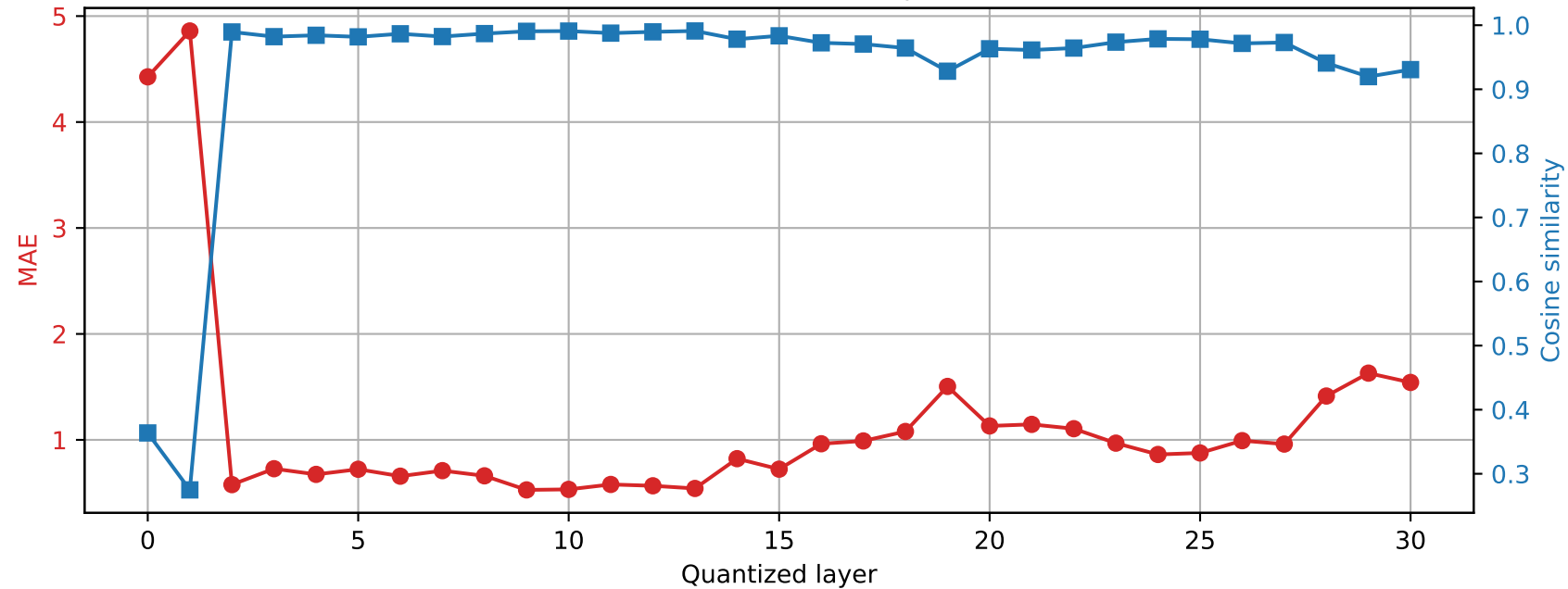
Mistral-7B-Instruct-v0.3 | Prompt 2 Final RMSNorm output damage | float64 → int2
