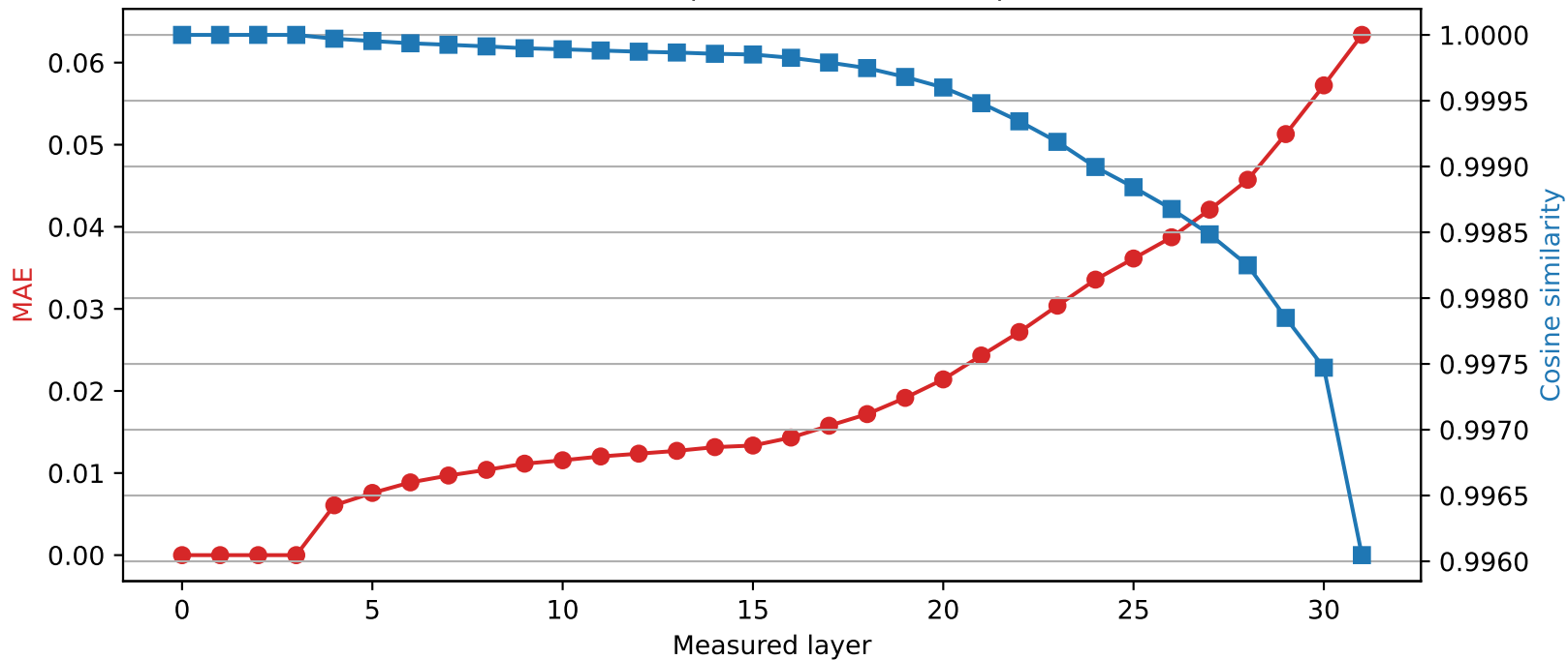
Mistral-7B-Instruct-v0.3 | Quantized layer 3 | float64 → int2
