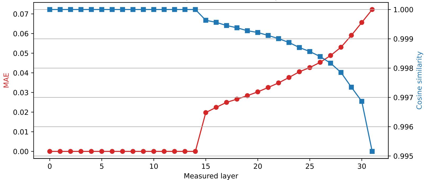
Mistral-7B-Instruct-v0.3 | Quantized layer 14 | float64 \rightarrow int2
