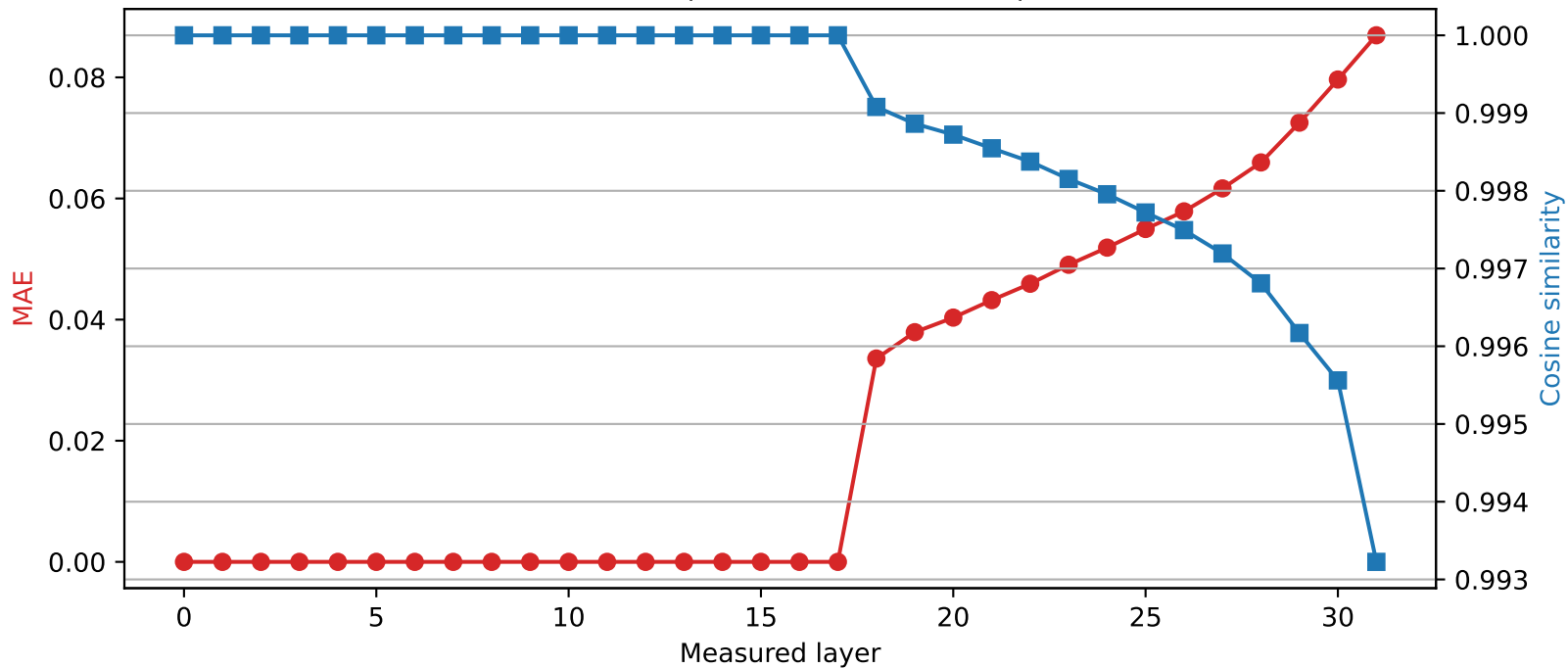
Mistral-7B-Instruct-v0.3 | Quantized layer 17 | float64 → int2
