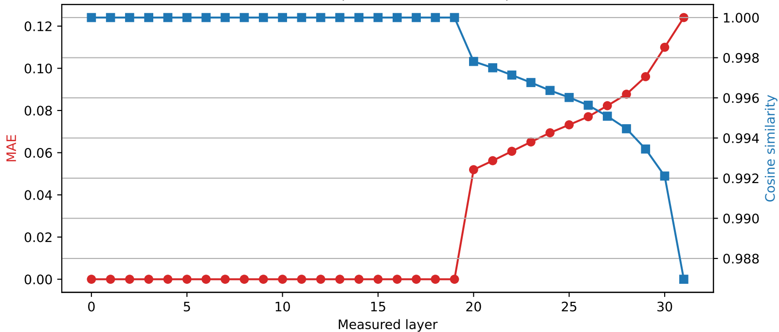
Mistral-7B-Instruct-v0.3 | Quantized layer 19 | float64 \rightarrow int2
