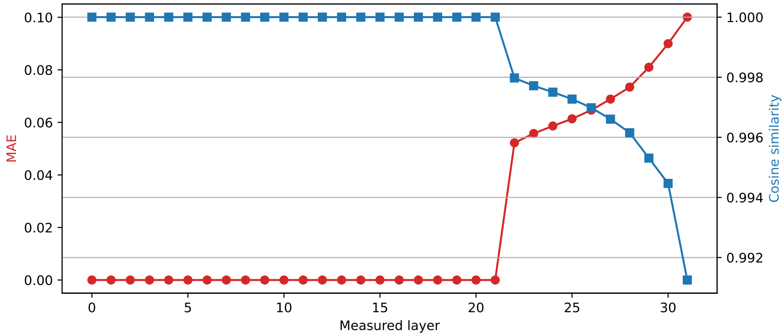
Mistral-7B-Instruct-v0.3 | Quantized layer 21 | float64 \rightarrow int2
