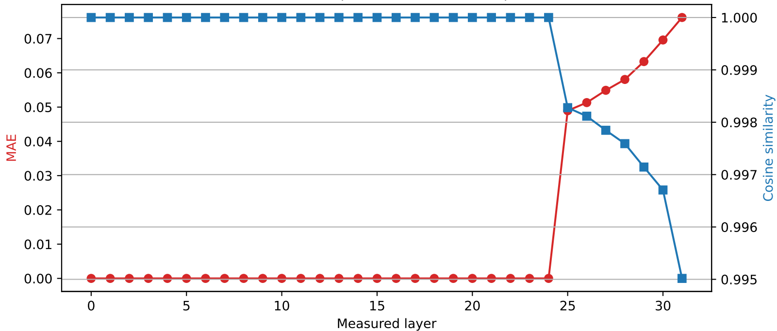
Mistral-7B-Instruct-v0.3 | Quantized layer 24 | float64 \rightarrow int2
