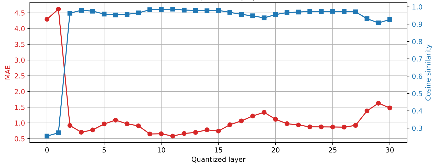
Mistral-7B-Instruct-v0.3 | Prompt 3 Final RMSNorm output damage | float64 \rightarrow int2
