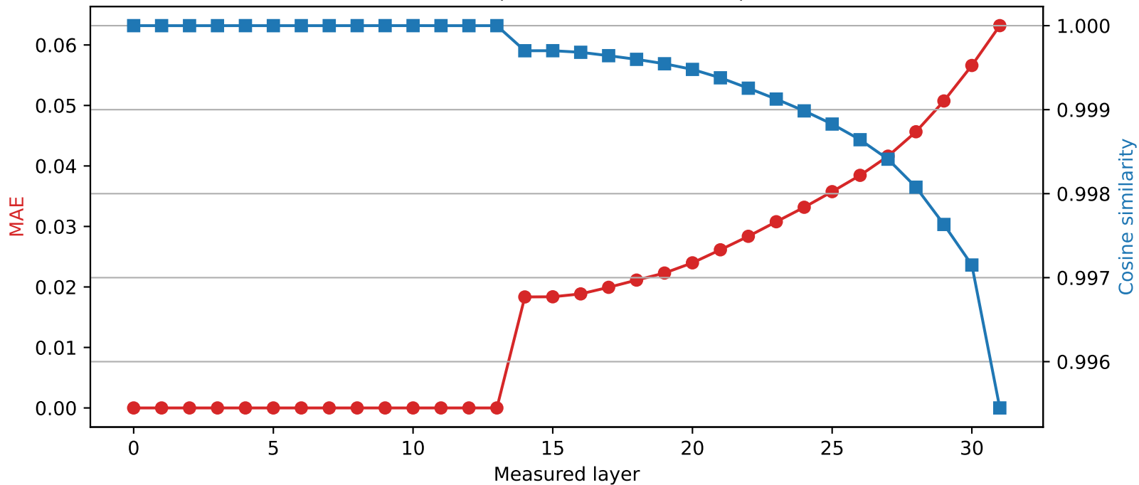
Mistral-7B-Instruct-v0.3 | Quantized layer 13 | float64 \rightarrow int2
