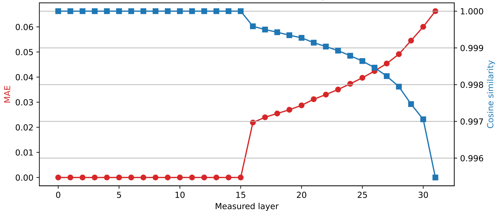
Mistral-7B-Instruct-v0.3 | Quantized layer 15 | float64 \rightarrow int2
