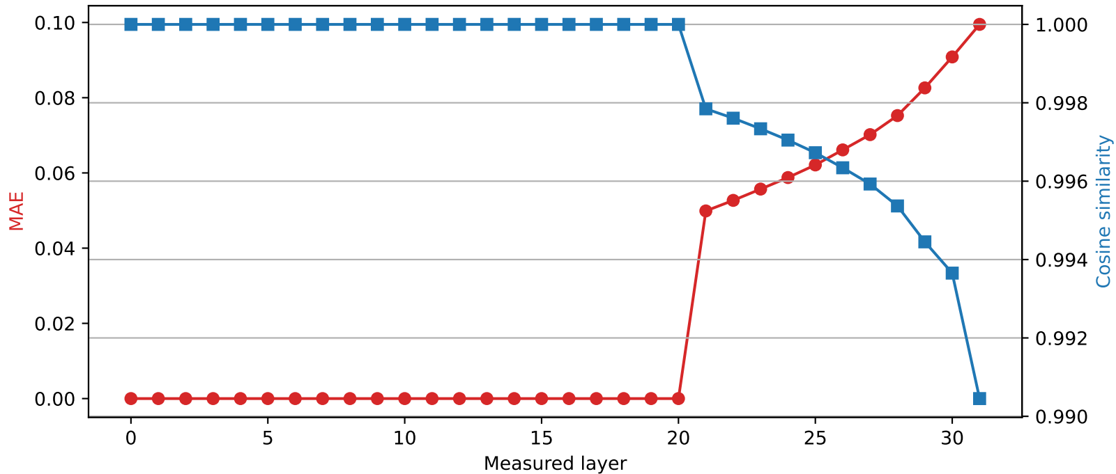
Mistral-7B-Instruct-v0.3 | Quantized layer 20 | float64 \rightarrow int2
