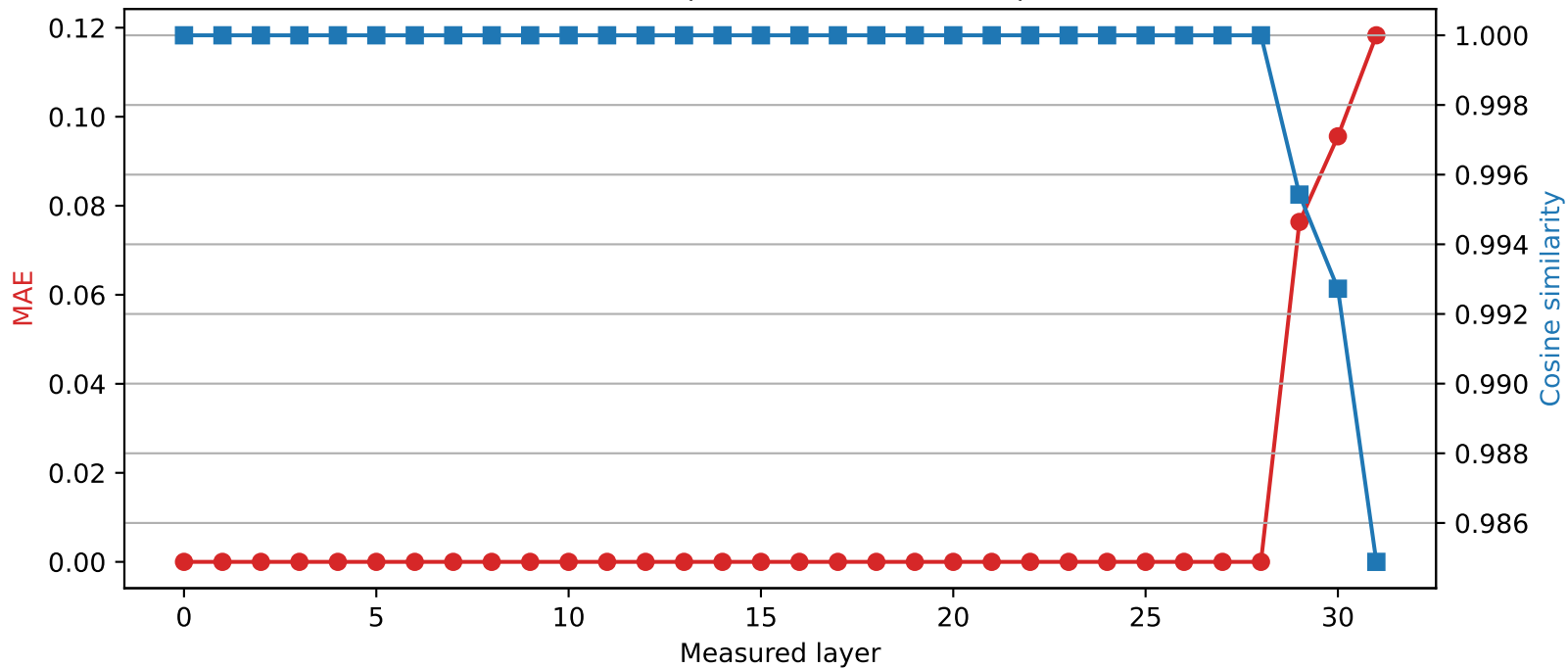
Mistral-7B-Instruct-v0.3 | Quantized layer 28 | float64 \rightarrow int2
