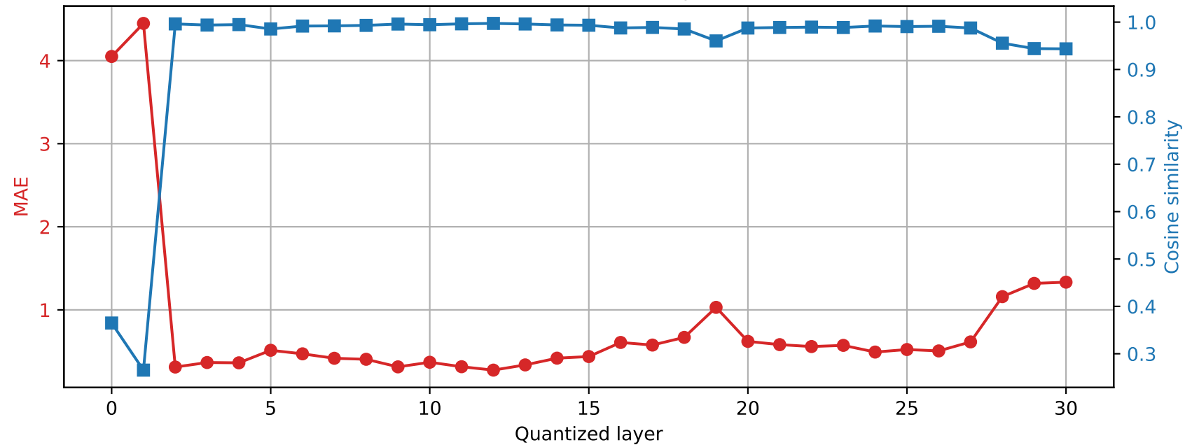
Mistral-7B-Instruct-v0.3 | Prompt 4 Final RMSNorm output damage | float64 \rightarrow int2
