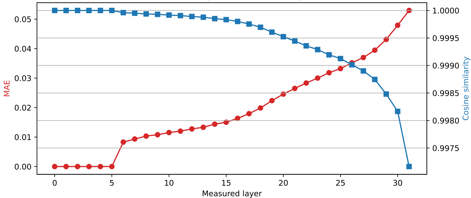
Mistral-7B-Instruct-v0.3 | Quantized layer 5 | float64 → int2
