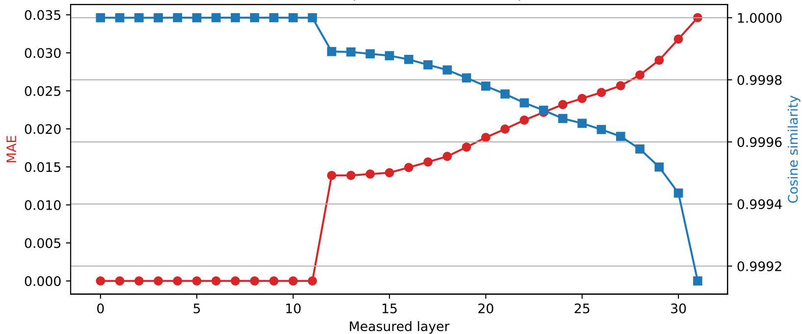
Mistral-7B-Instruct-v0.3 | Quantized layer 11 | float64 \rightarrow int2
