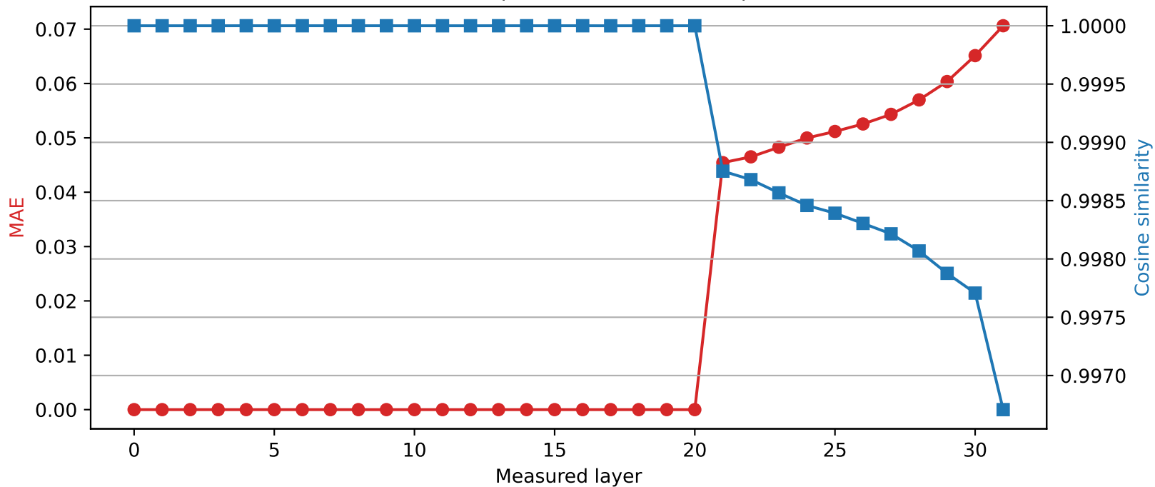
Mistral-7B-Instruct-v0.3 | Quantized layer 20 | float64 → int2
