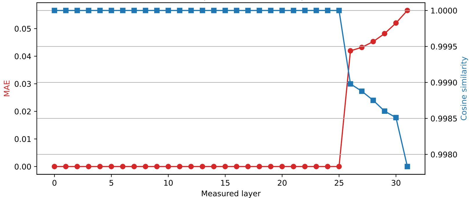
Mistral-7B-Instruct-v0.3 | Quantized layer 25 | float64 → int2
