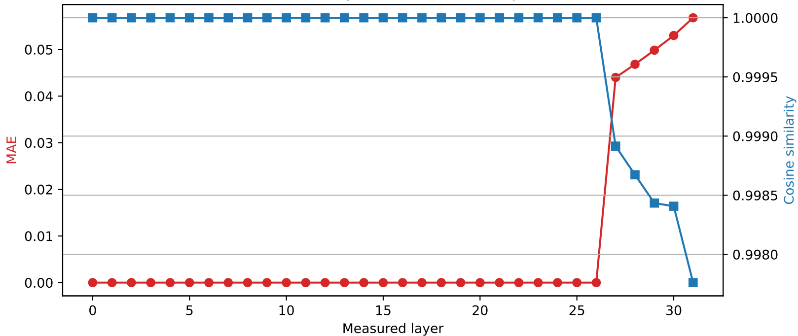
Mistral-7B-Instruct-v0.3 | Quantized layer 26 | float64 \rightarrow int2
