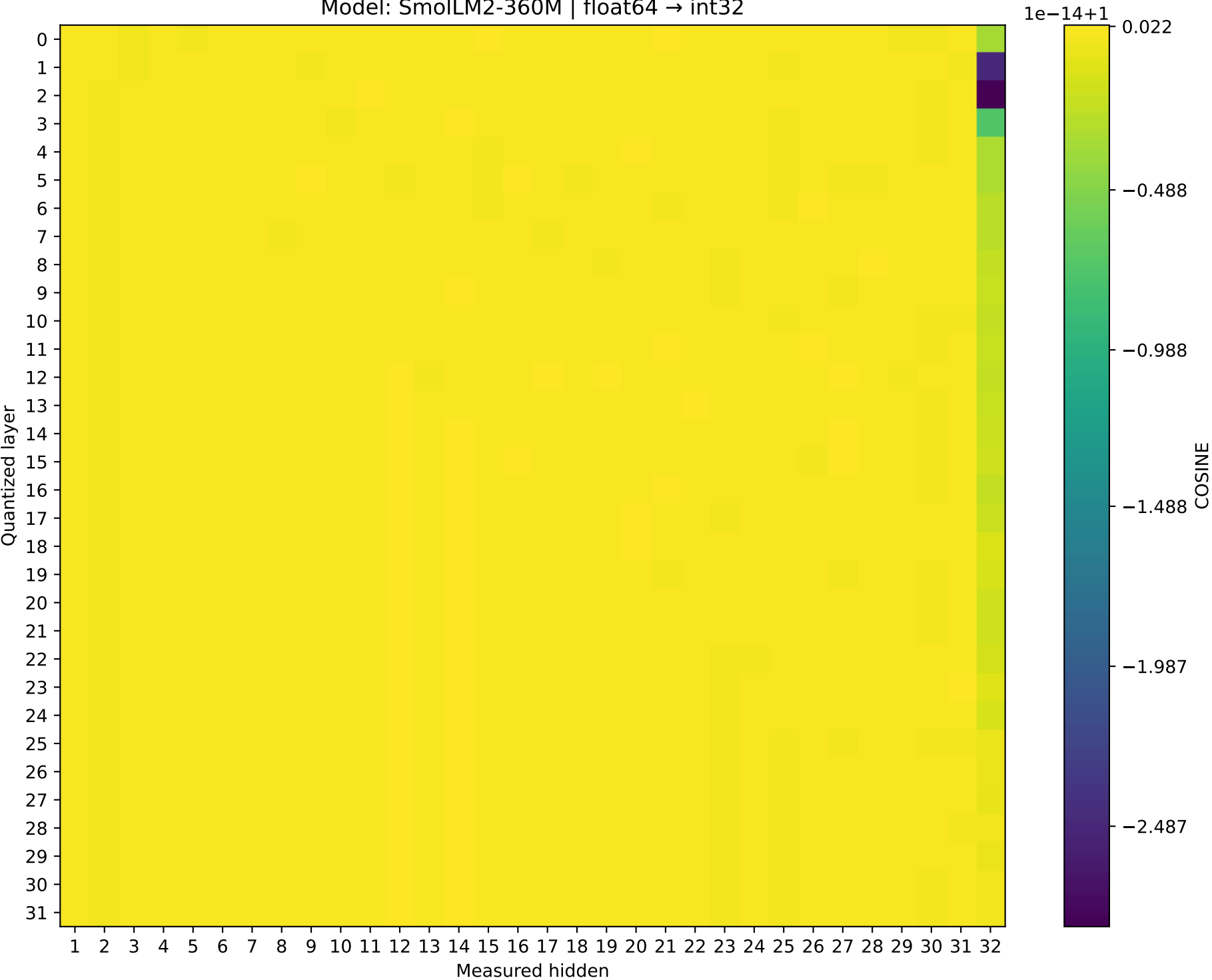
Model: SmolLM2-360M | float64 → int32
