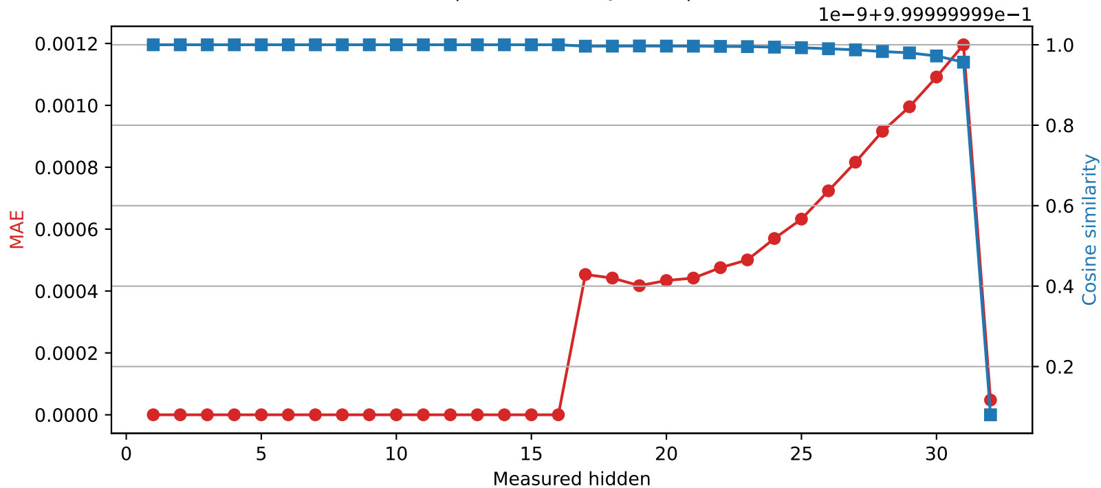
SmolLM2-360M | Quantized layer 16 | float32 → int16
