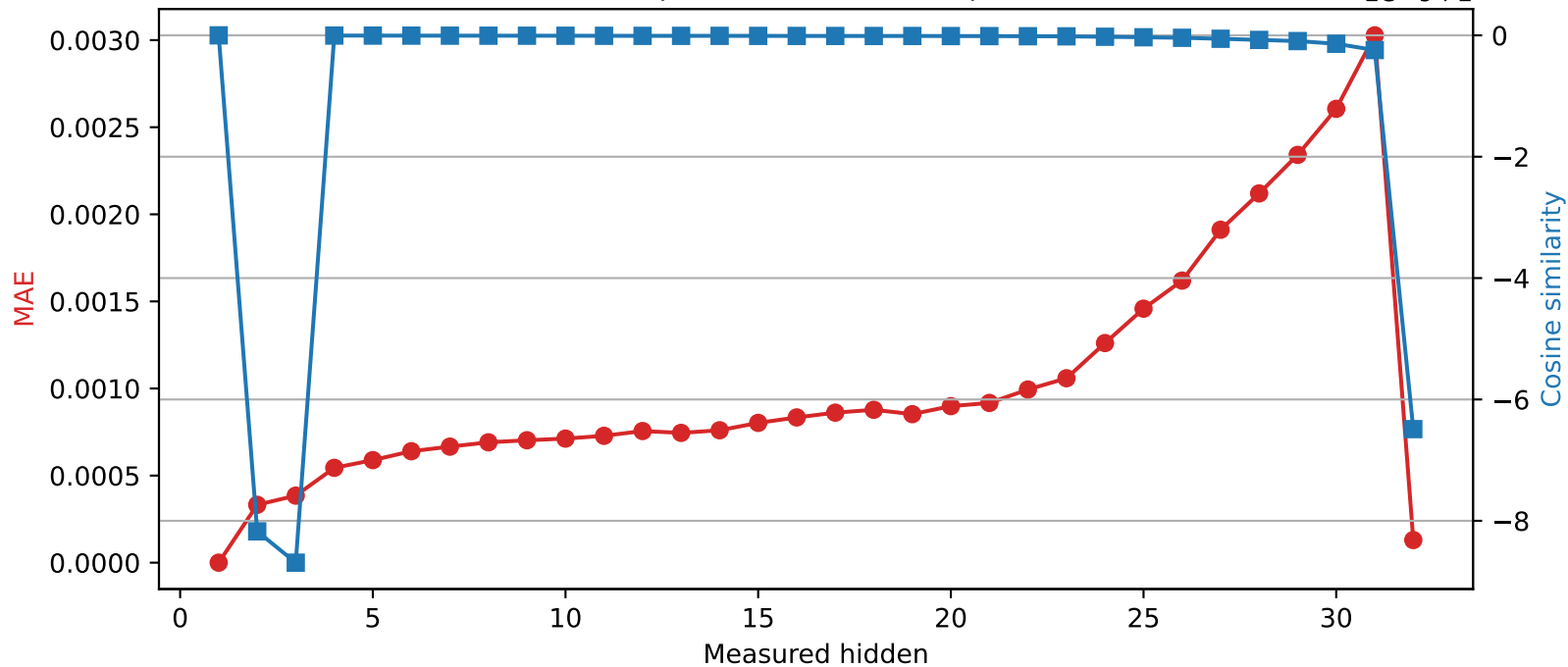
SmolLM2-360M | Quantized layer 1 | float32 → int16
