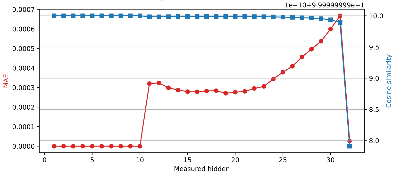
SmolLM2-360M | Quantized layer 10 | float32 → int16
