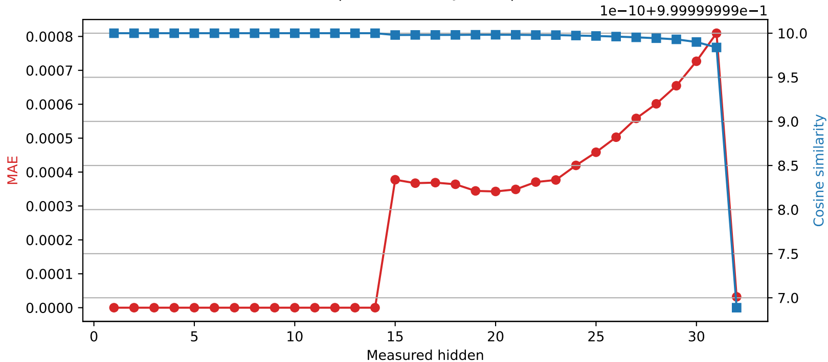
SmolLM2-360M | Quantized layer 14 | float32 → int16
