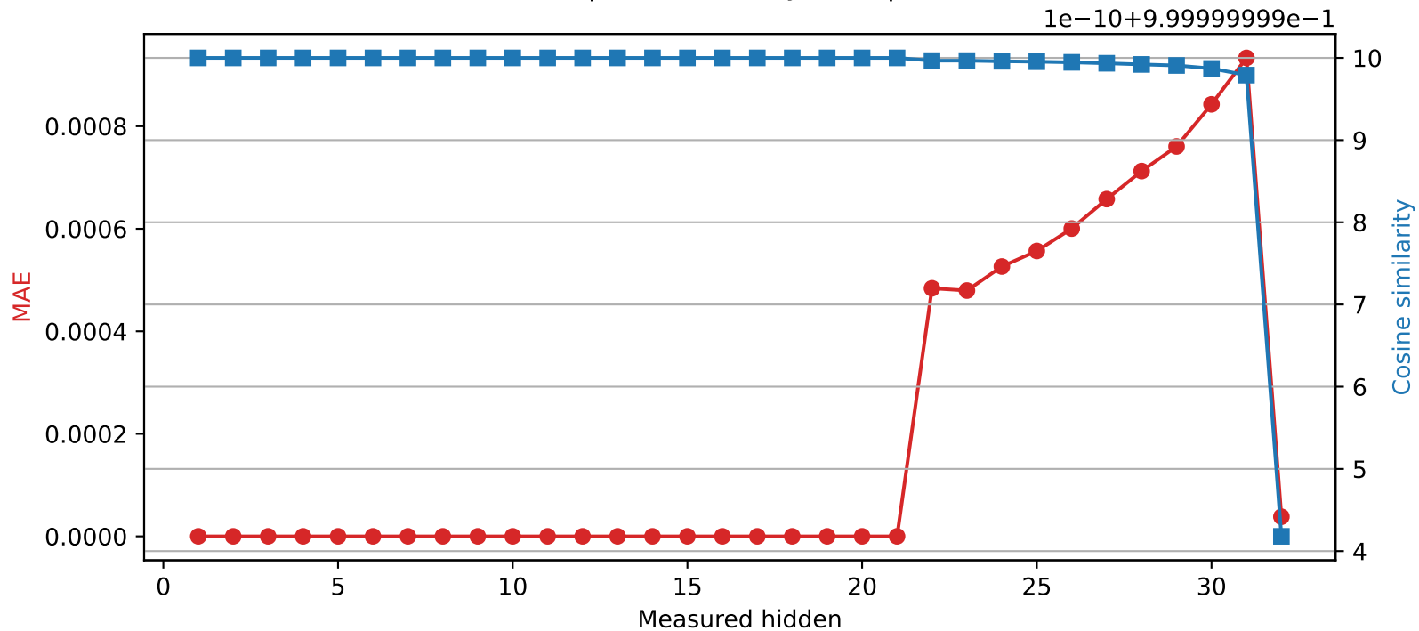
SmolLM2-360M | Quantized layer 21 | float32 → int16
