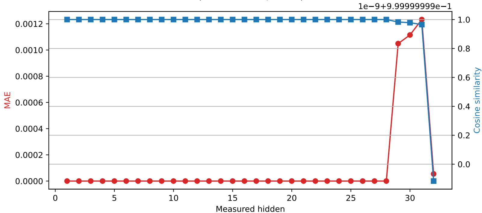
SmolLM2-360M | Quantized layer 28 | float32 → int16
