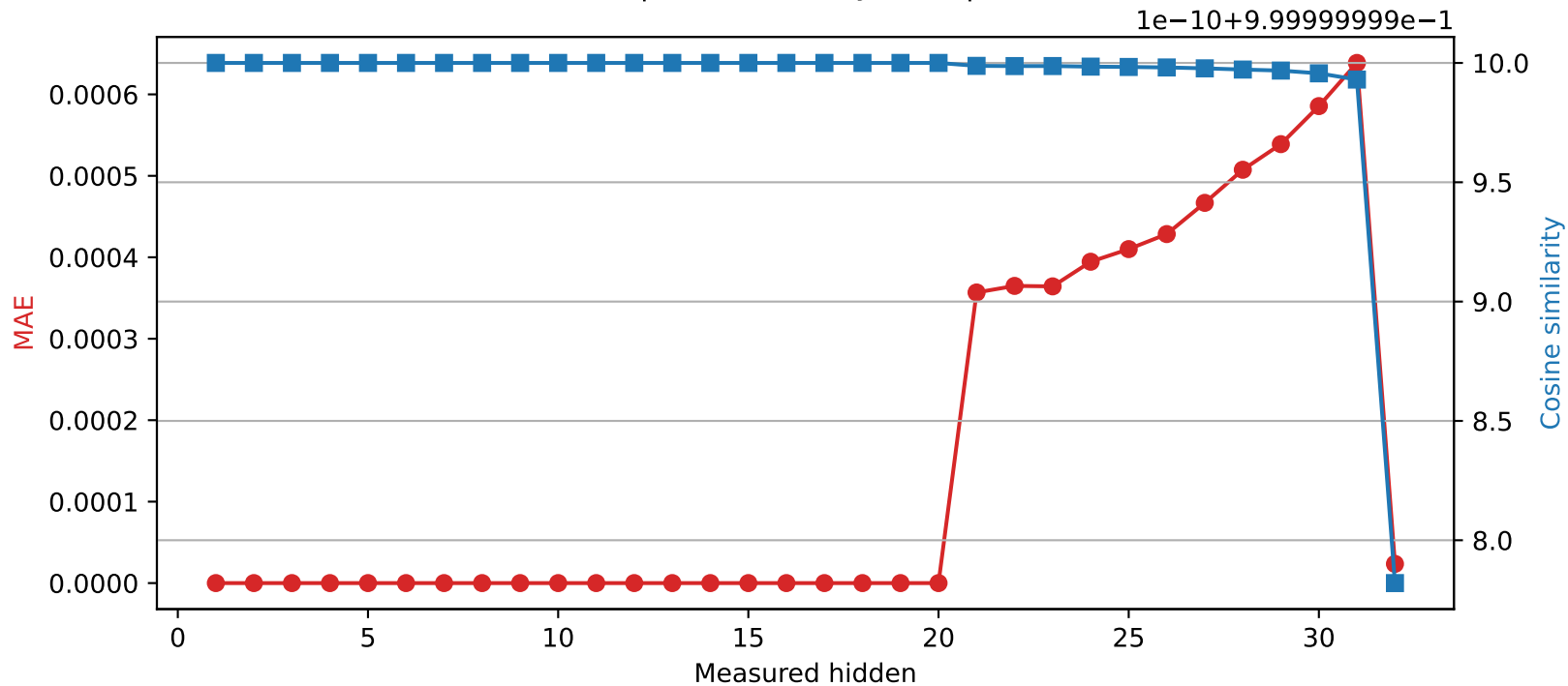
SmolLM2-360M | Quantized layer 20 | float32 → int16
