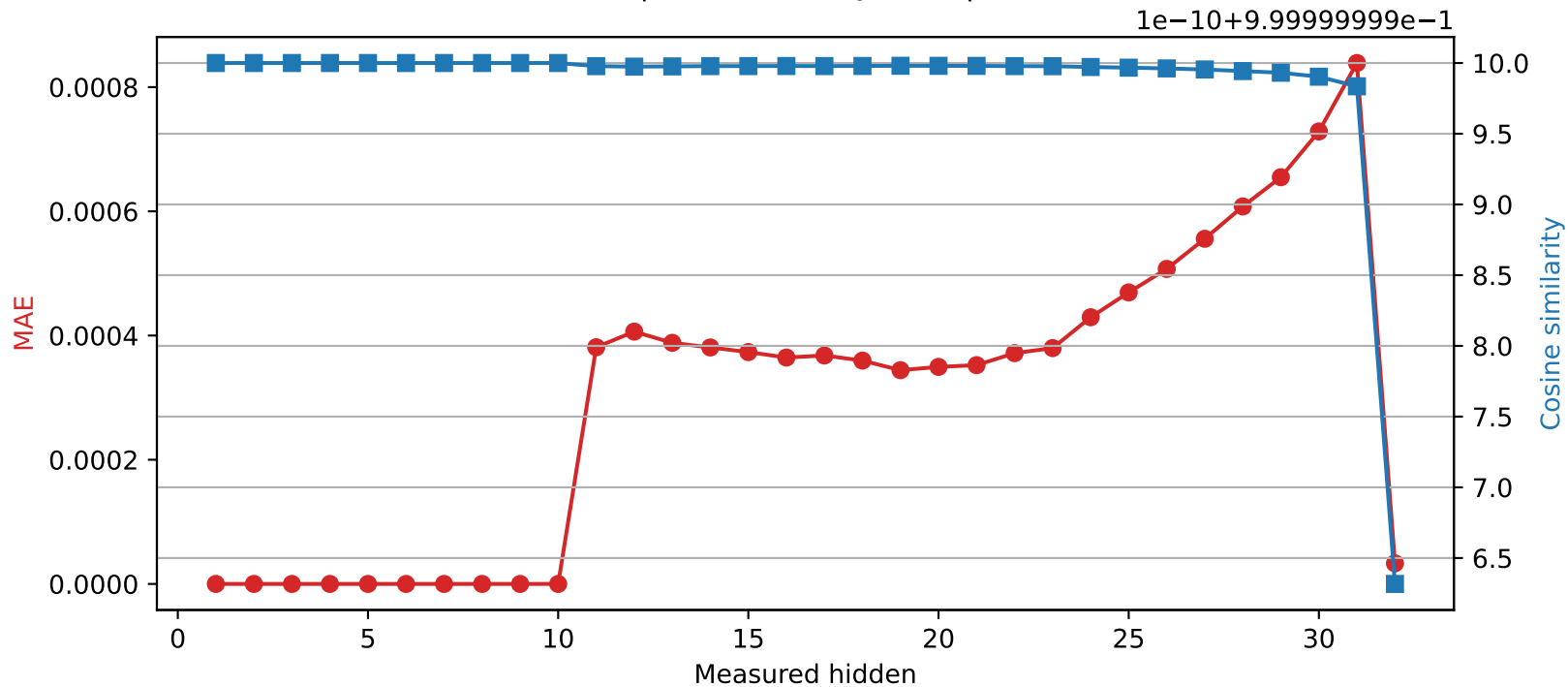
SmolLM2-360M | Quantized layer 10 | float64 → int16
