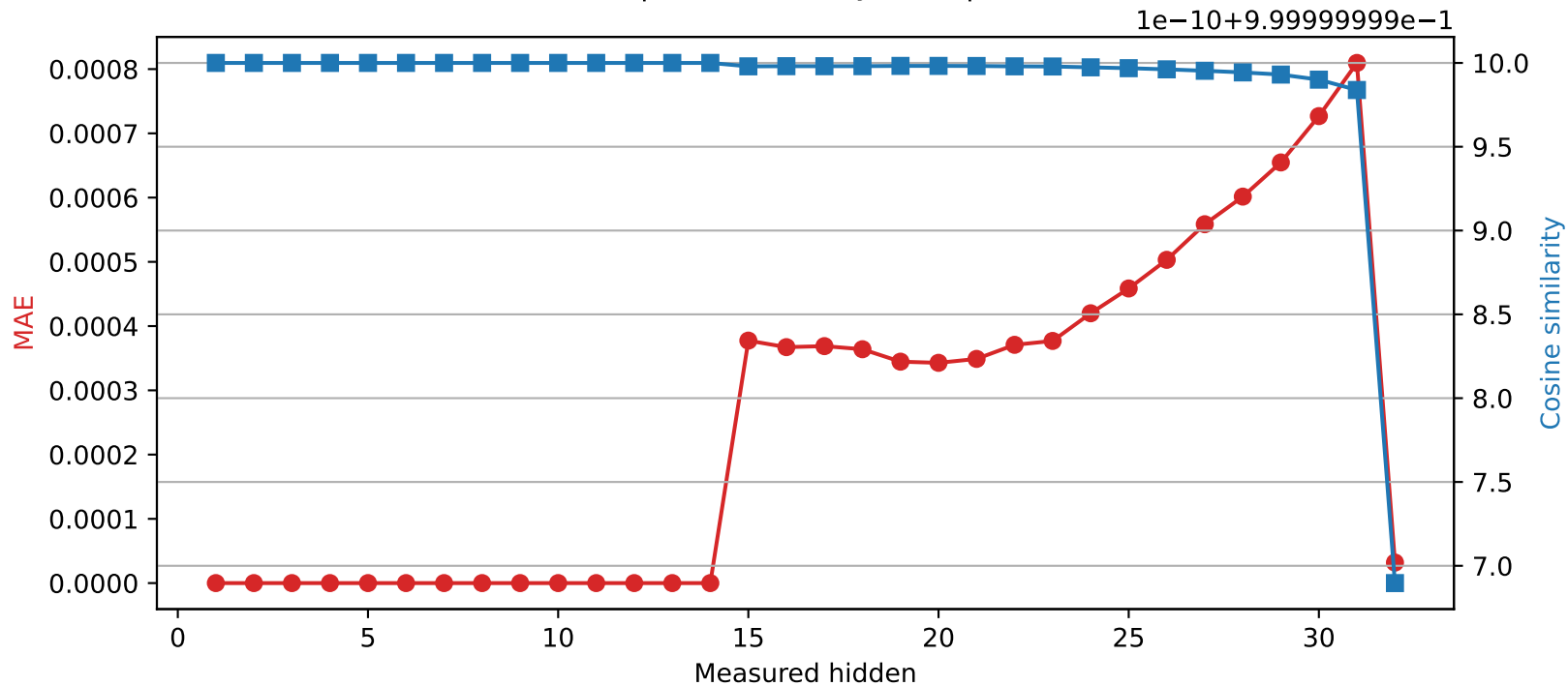
SmolLM2-360M | Quantized layer 14 | float64 → int16
