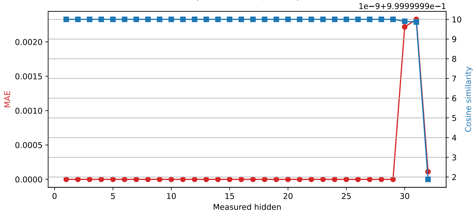
SmolLM2-360M | Quantized layer 29 | float64 → int16
