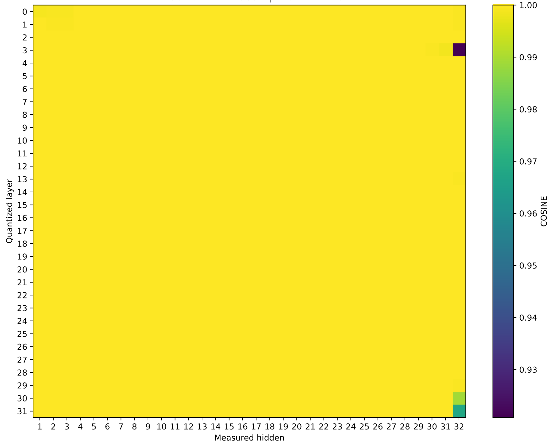
Model: SmolLM2-360M | float16 → int8
