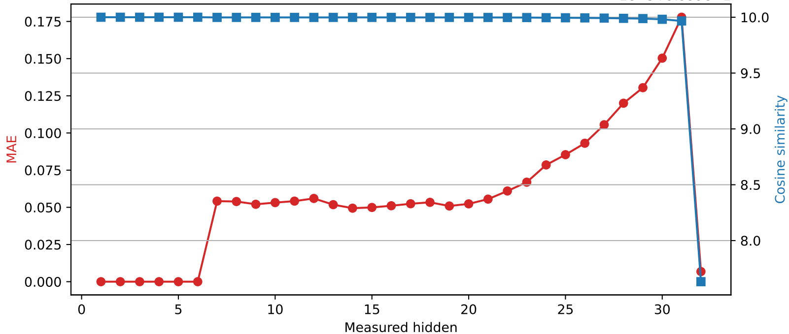
SmolLM2-360M | Quantized layer 6 | float16 \rightarrow int8 1e-5+9.999e-1
