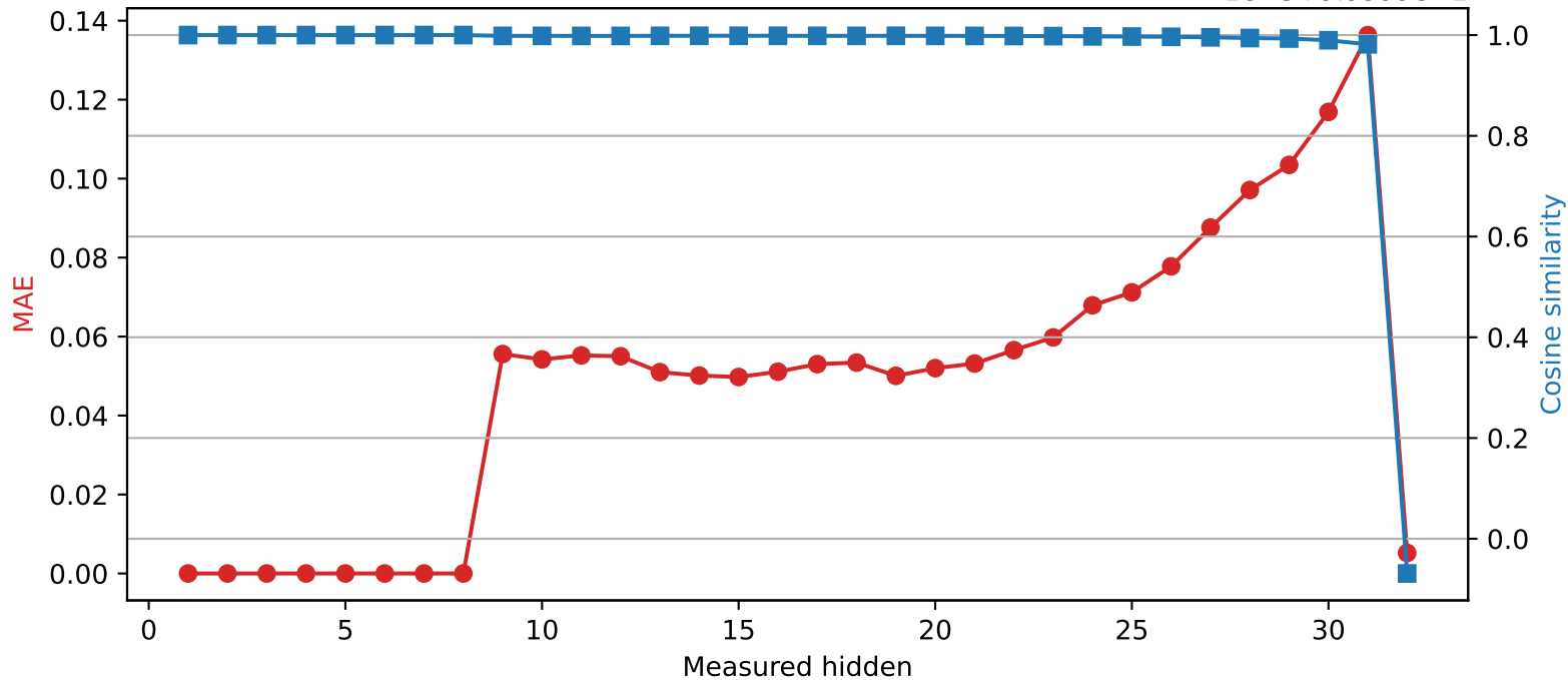
SmolLM2-360M | Quantized layer 8 | float16 \rightarrow int8 1e-5+9.9999e-1
