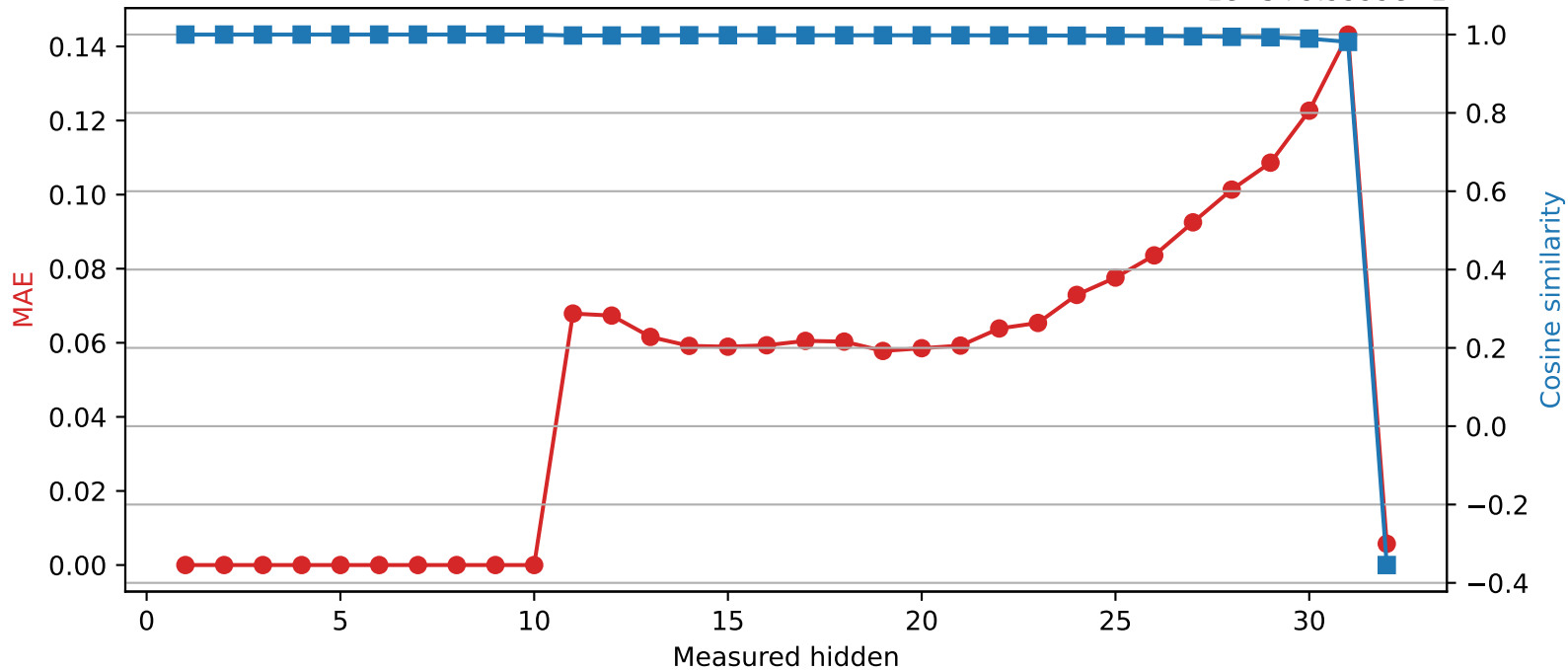
SmolLM2-360M | Quantized layer 10 | float16 \rightarrow int8 1e-5+9.9999e-1
