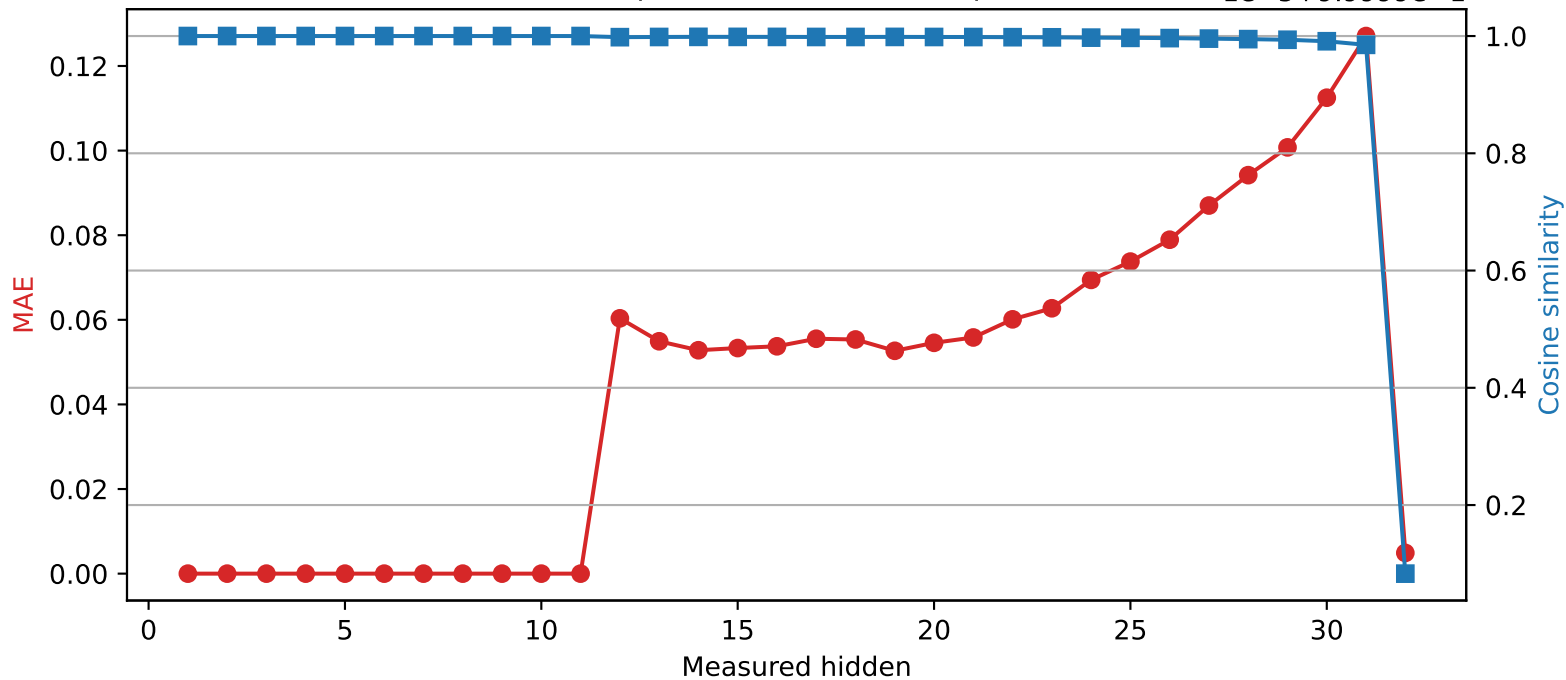
SmolLM2-360M | Quantized layer 11 | float16 \rightarrow int8 1e-5+9.9999e-1
