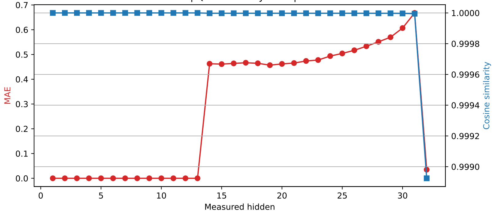
SmolLM2-360M | Quantized layer 13 | float16 \rightarrow int8
