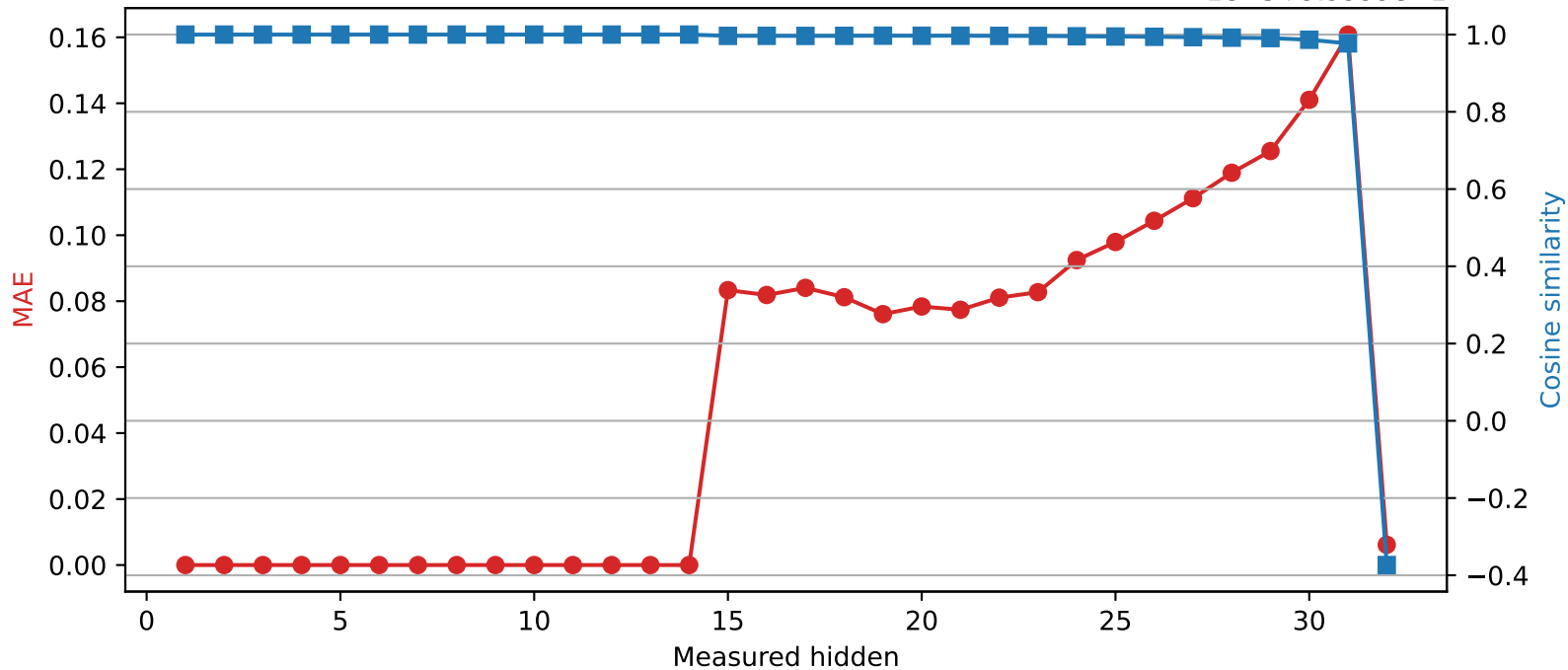
SmolLM2-360M | Quantized layer 14 | float16 \rightarrow int8 1e-5+9.9999e-1
