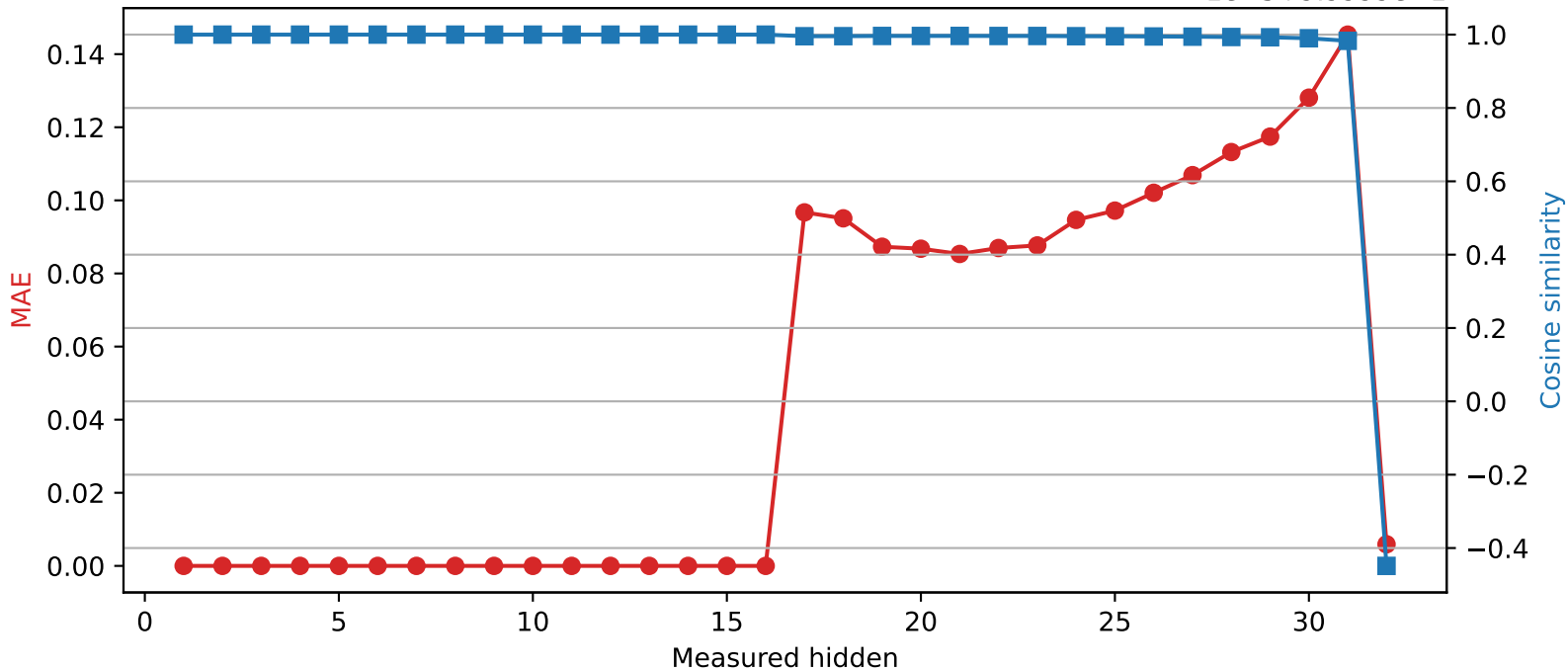
SmolLM2-360M | Quantized layer 16 | float16 \rightarrow int8 1e-5+9.9999e-1
