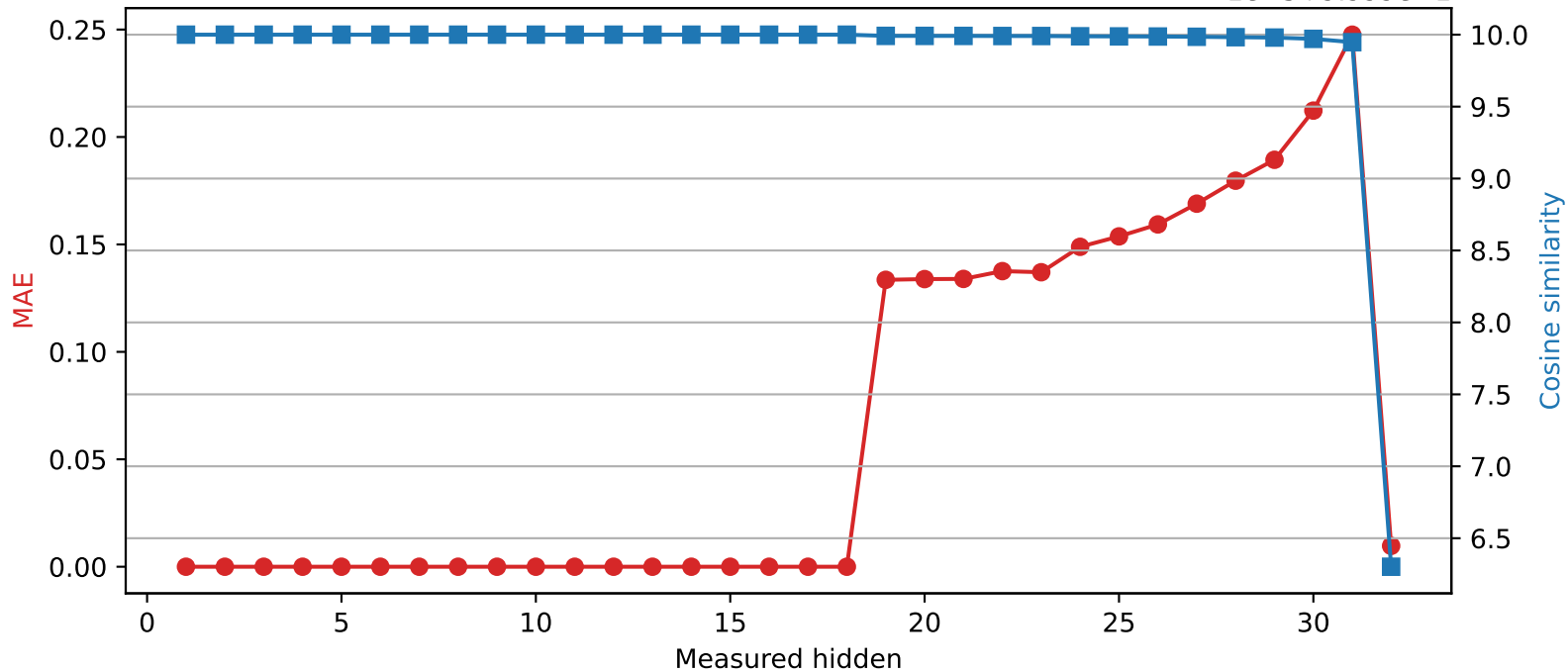
SmolLM2-360M | Quantized layer 18 | float16 → int8 1e-5 + 9.999e-1
