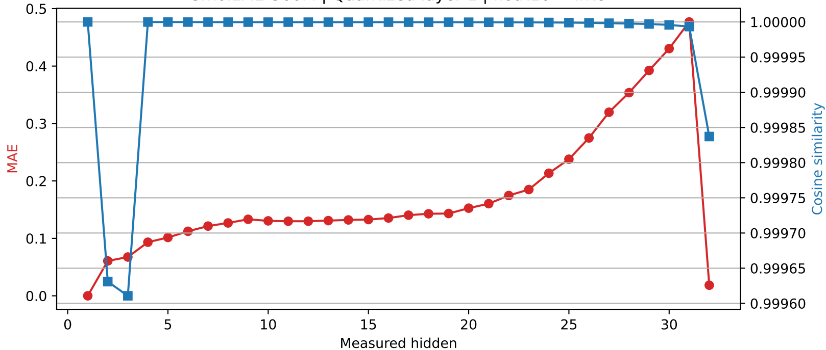
SmolLM2-360M | Quantized layer 1 | float16 → int8
