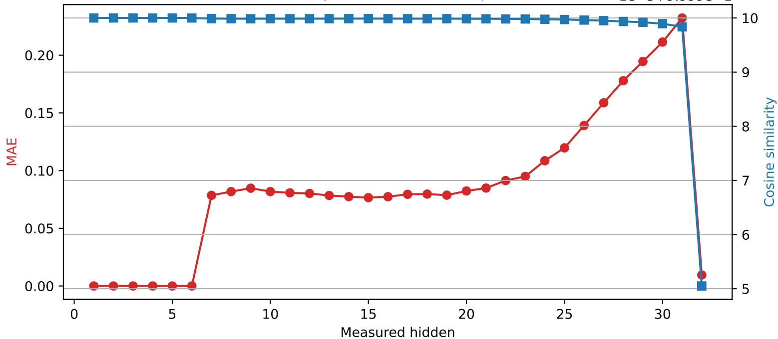
SmolLM2-360M | Quantized layer 6 | float16 → int8
