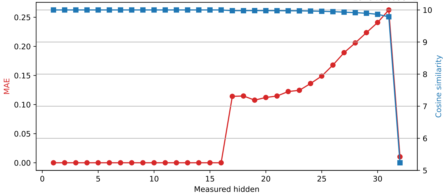
SmolLM2-360M | Quantized layer 16 | float16 \rightarrow int8 1e-5+9.999e-1
