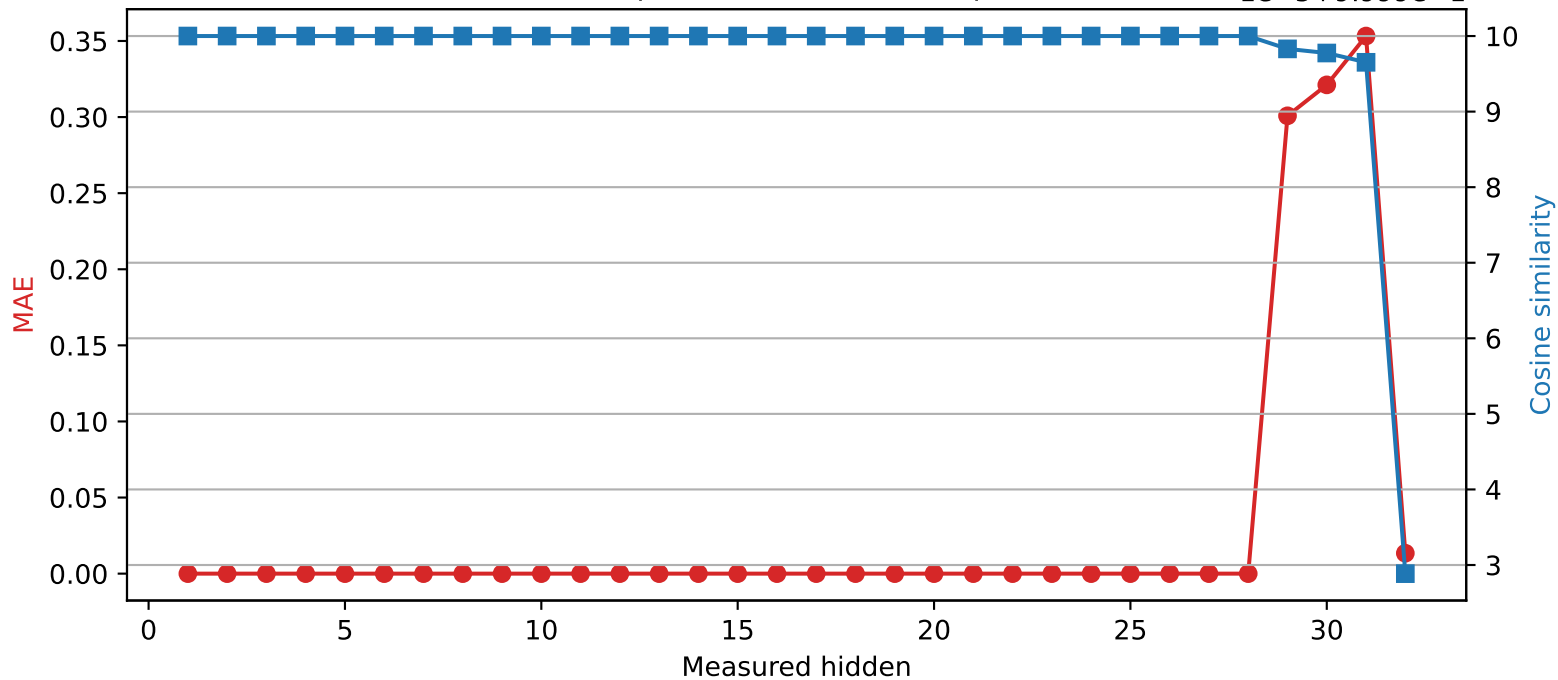
SmolLM2-360M | Quantized layer 28 | float16 → int8
