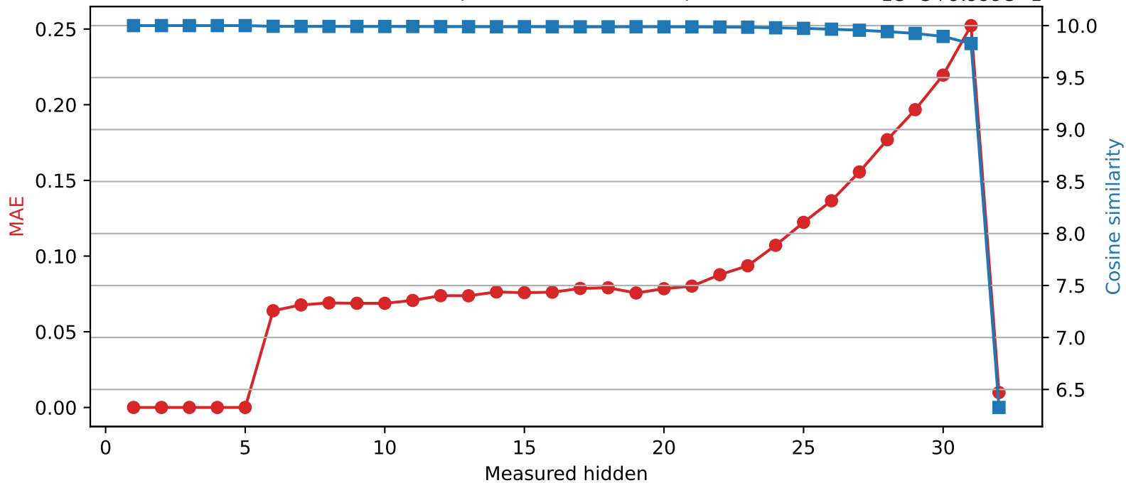
SmolLM2-360M | Quantized layer 5 | float16 → int8
