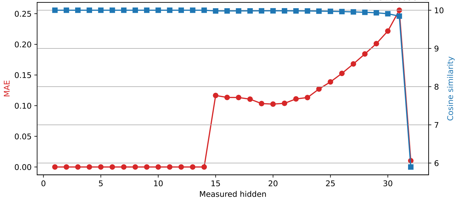
SmolLM2-360M | Quantized layer 14 | float16 → int8 1e-5 + 9.999e-1
