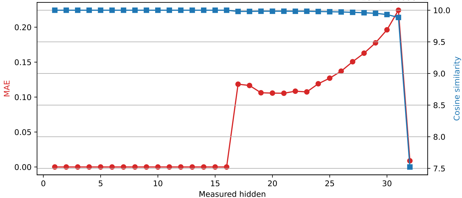
SmolLM2-360M | Quantized layer 16 | float16 → int8 1e-5 + 9.999e-1
