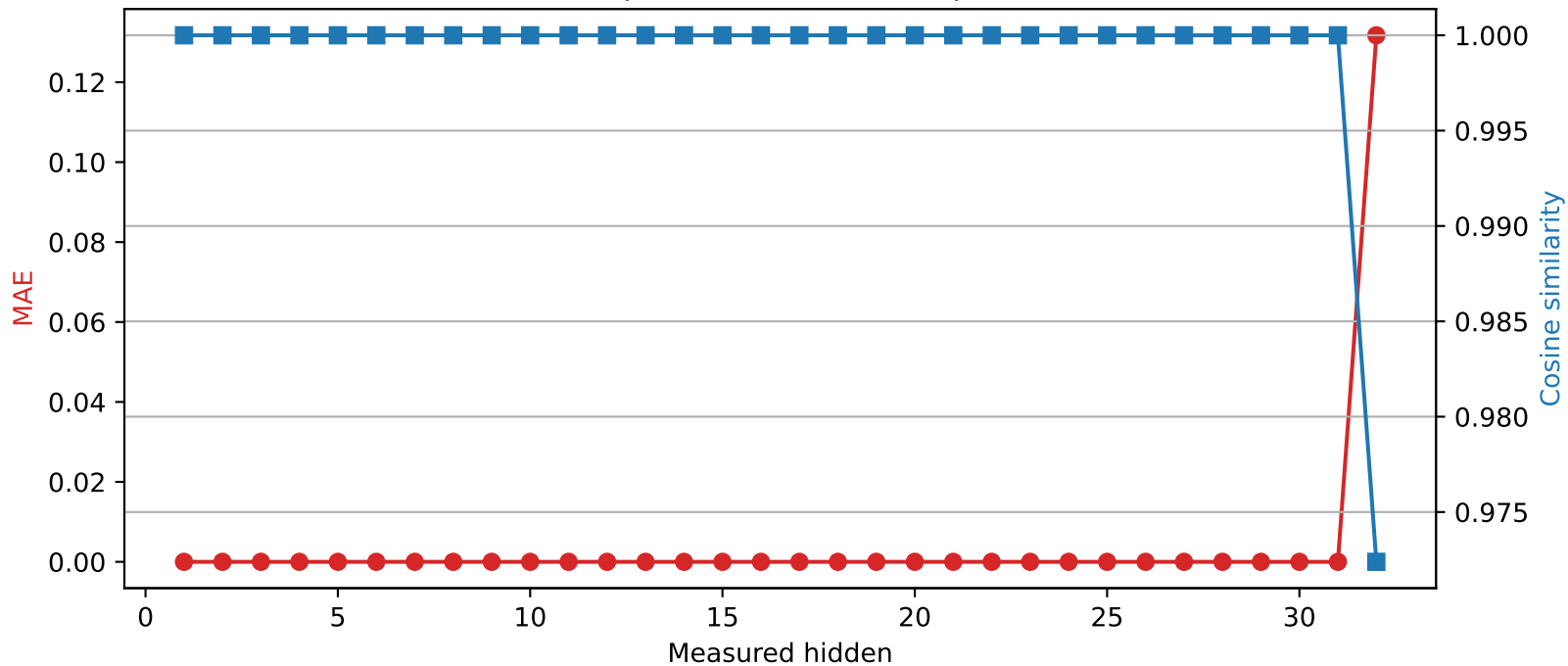
SmolLM2-360M | Quantized layer 31 | float16 \rightarrow int8
