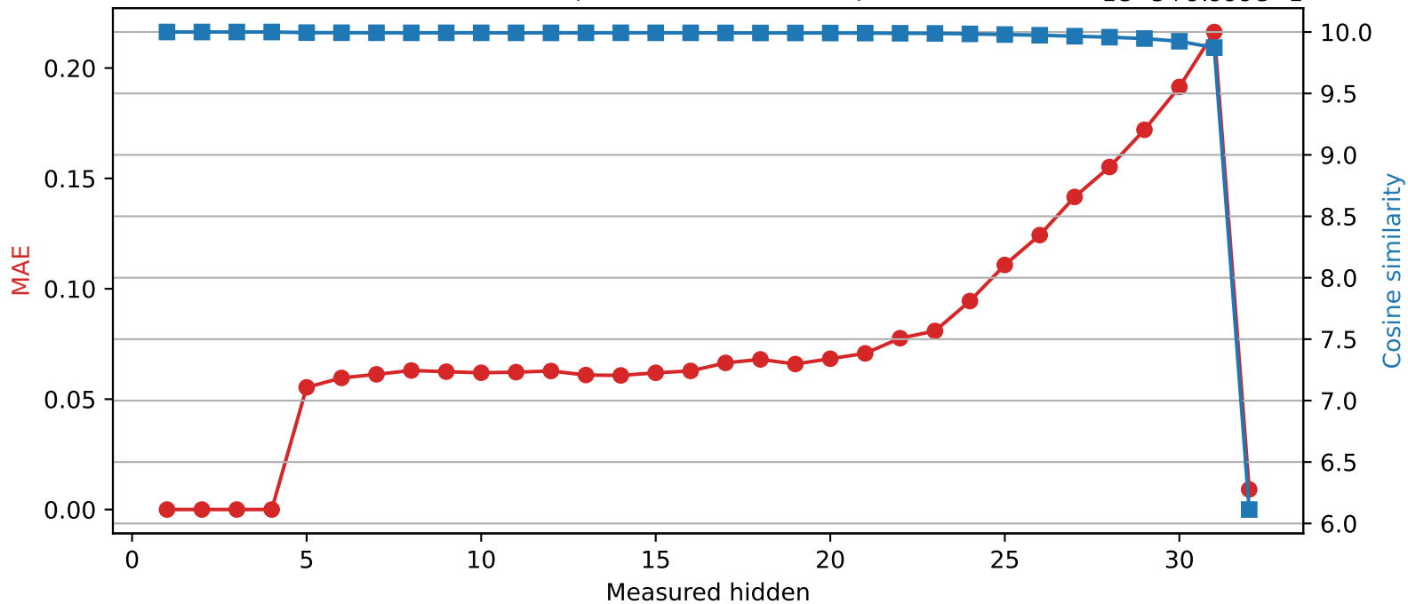
SmolLM2-360M | Quantized layer 4 | float16 → int8
